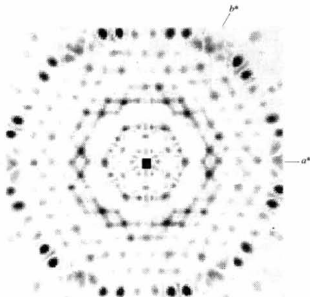
Fig. 7. Simulated pattern corresponding to Fig. 2. On the periphery, the circle of intense reflections corresponds to the (hk1) plane.
